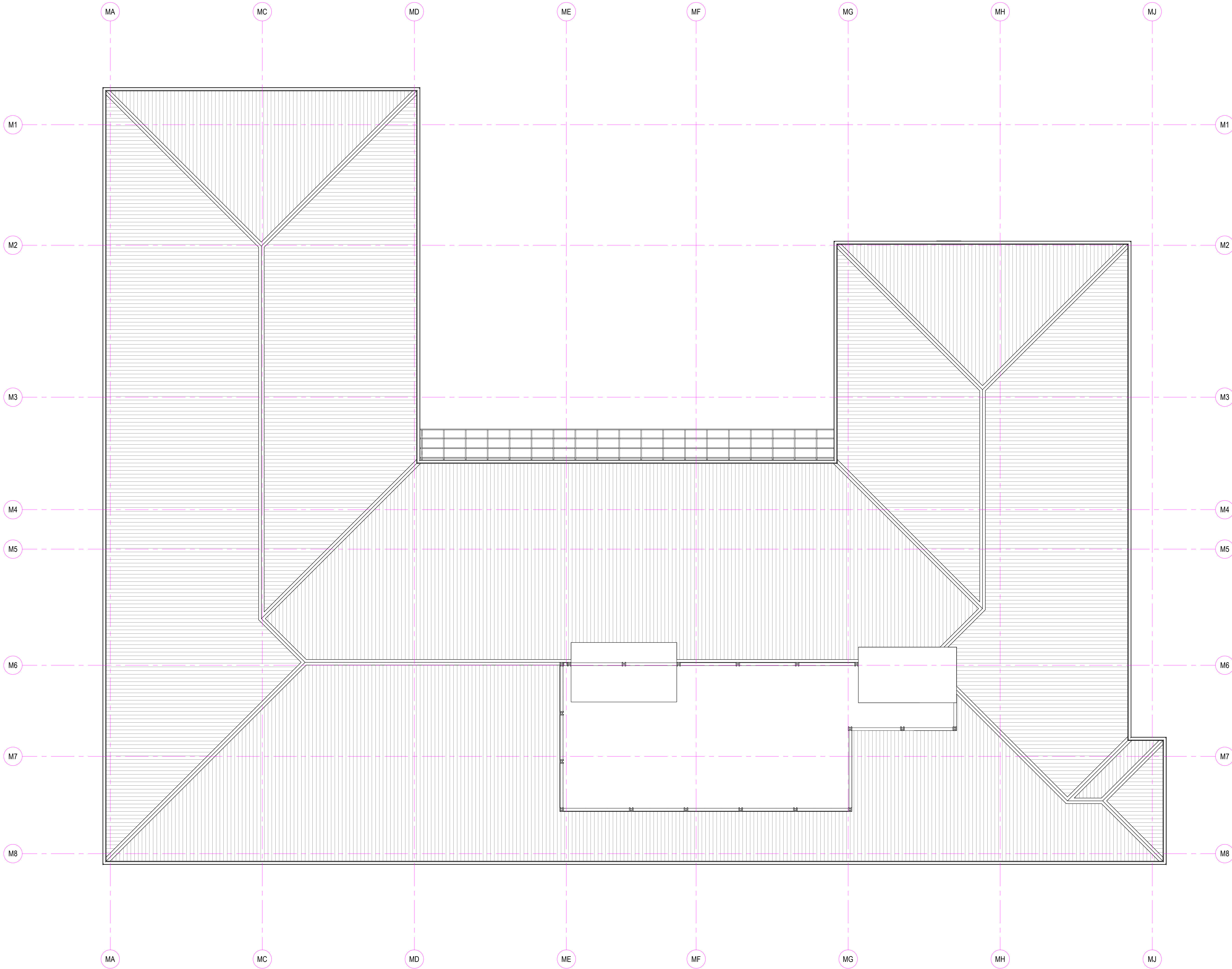
6 ROOF PLAN Scale 1 : 100
